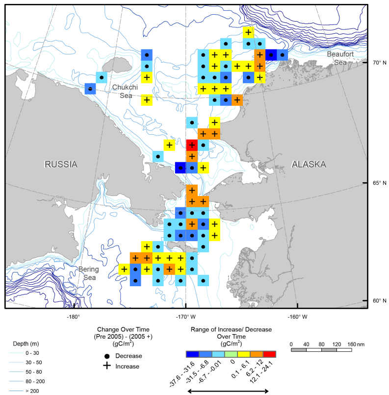
Figure C3.5 Distribution of gridded benthic station biomass data (gC/m 2 ) for period pre-2005 and post-2005.
