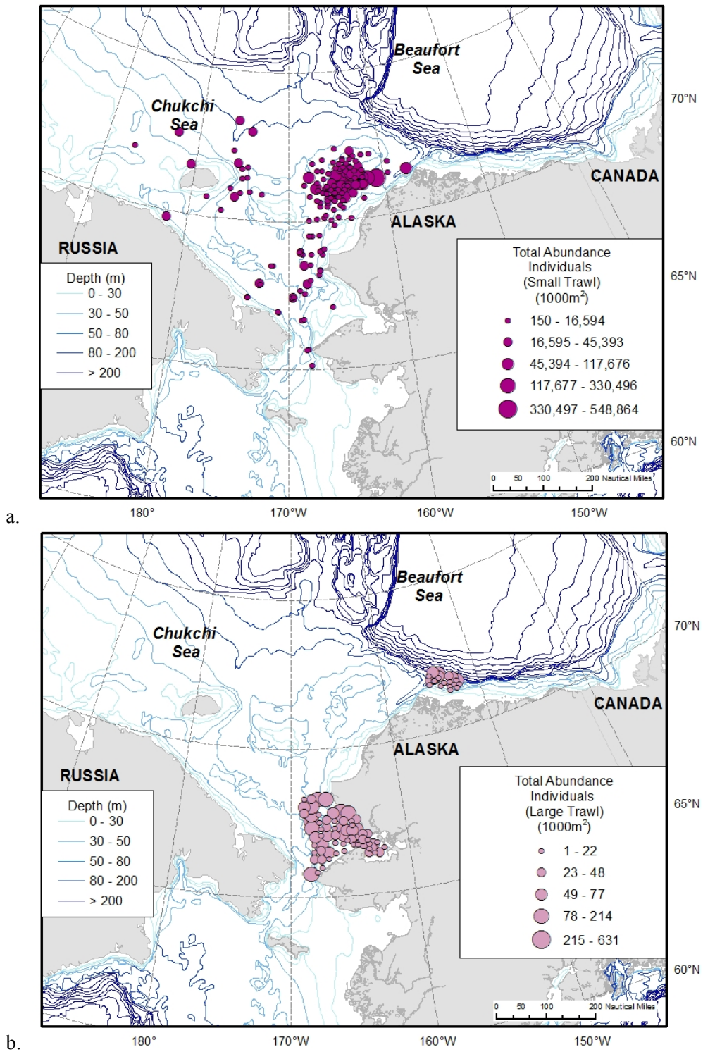
Figure C4.3 Distribution of epifaunal abundance from a. small mesh nets, and b. large mesh nets. Jenks natural breaks classification was used to group the data. Data sources listed in Table B4.1.
