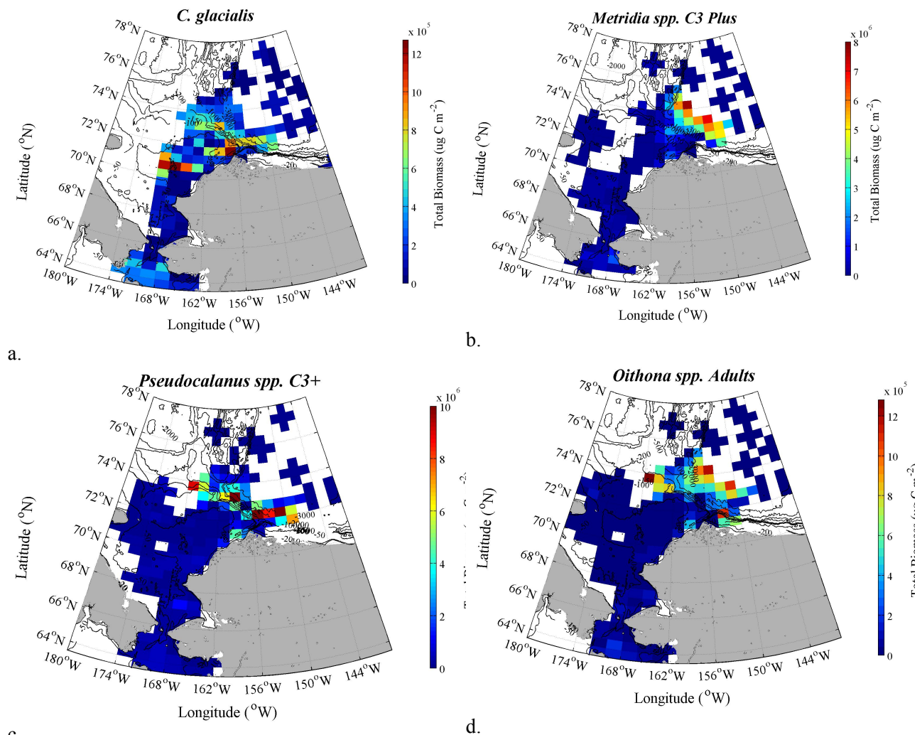
Figure C2.13 Integrated (surface to bottom or 100 m in deeper water) water column biomass ( \mu\text{g carbon m}^{-2} ) of a. Calanus glacialis/marshallae (C1-adult), b. Metridia spp. (C3-adult), c. Pseudocalanus spp. (C3-adult), and d. Oithona similis (adult only) during summer (July-September).
