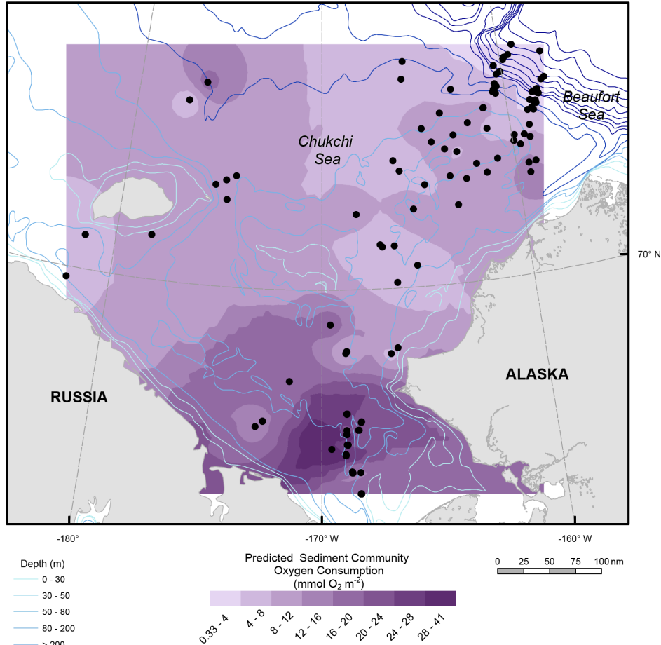
Figure 3.9. Distribution of sediment community oxygen consumption ( \text{mmol O}_2/\text{m}^2/\text{d} ) from 2000-2012 in the Chukchi Sea (updated from Mathis et al. 2014).
