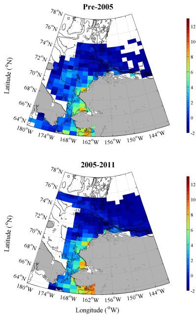
Figure C2.2 Bottom temperature during the summer (July-September) pre- 2005 (left top) and 2005-2011 (left bottom). File=Summer_BotT_TwoPeriods.jpg.
