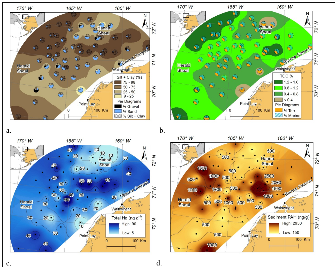
Figure C6.1 Contour maps for surface sediment (a) grain size, (b) total organic carbon (TOC) and % terrestrial and marine OC based on data for \delta^{13}\text{C} , (c) total mercury and (d) total polycyclic aromatic hydrocarbons (TPAH) in the northeastern Chukchi Sea.
