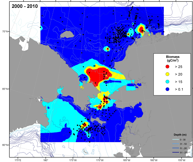
Figure C3.4 Distribution of station macrofaunal biomass over the 2000-2010 period showing persistent hotspots of benthic macrofaunal biomass.
