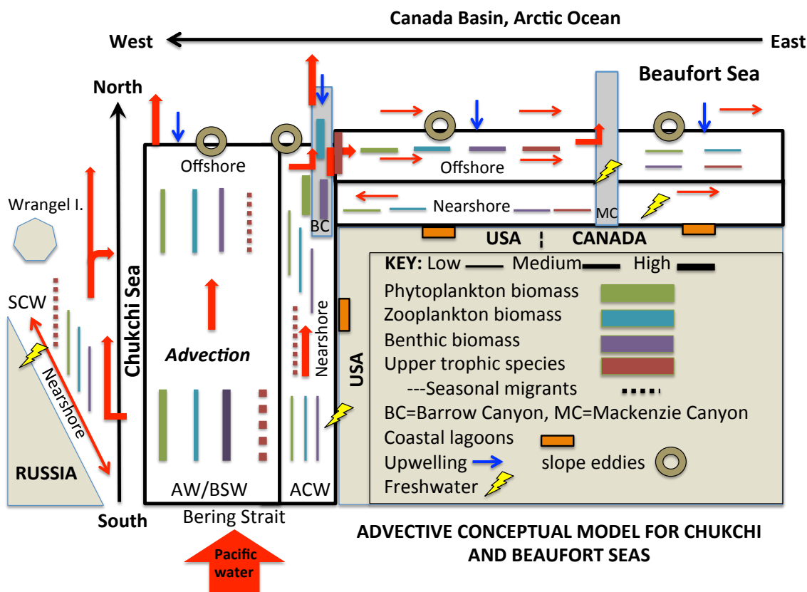
Figure D1. Advective conceptual model for the Chukchi and Beaufort seas in the Pacific Arctic region. The Pacific water advected northward through Bering Strait (large red arrow) includes all physical, chemical and biological components from the northern Bering Sea as an "input function" to this model. AW/BSW=Anadyr Water/Bering Shelf Water; ACW=Alaska Coastal Water; and SCW=Siberian Coastal Water. The model has an offshore and nearshore component; the latter considered being <20 nautical miles from the Alaskan, Canadian and Russian coasts. The smaller red arrows indicate the advection of Pacific water in the downstream portions of the ecosystem. Other components of the model are identified in the "key" within the figure and explained further in the text below.
