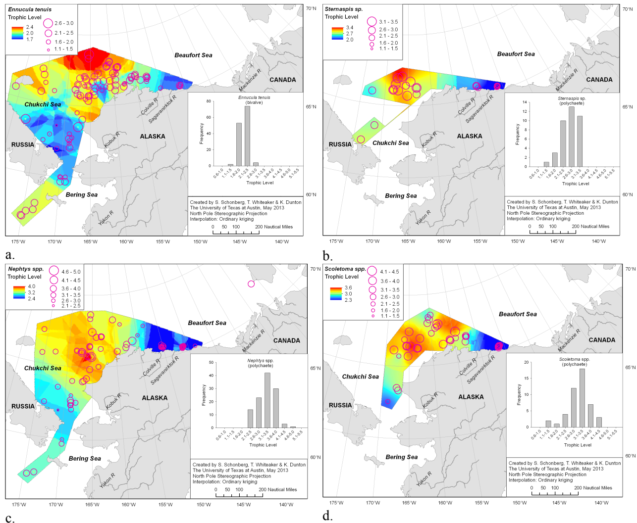
Figure C5.8 Variation in trophic level for infaunal consumers, including a. Ennucula tenuis (bivalve), b. Sternaspis sp. (polychaete), c. Nephtys spp. (polychaete), and d. Scoletoma (polychaete). Frequency distribution of predicted trophic level based on \delta^{15}\text{N} analyses depicted in lower right inset.
